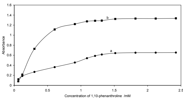
Figure 4. Effect of 1,10-phenanthroline concentration on the absorbance of the ferriox produced from the oxidation of (a) paracetamol and (b) salicylamide with \text{Fe}^{3+} . Conditions: salicylamide, 20 \mu\text{g mL}^{-1} ; paracetamol, 5.0 \mu\text{g mL}^{-1} ; pH, 4.5; \text{Fe}^{3+} , 6.45 \times 10^{-4} M; T = 60^\circ\text{C} .
